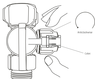
Figure 3 - SmartTee™ Quick Connect Fitting
