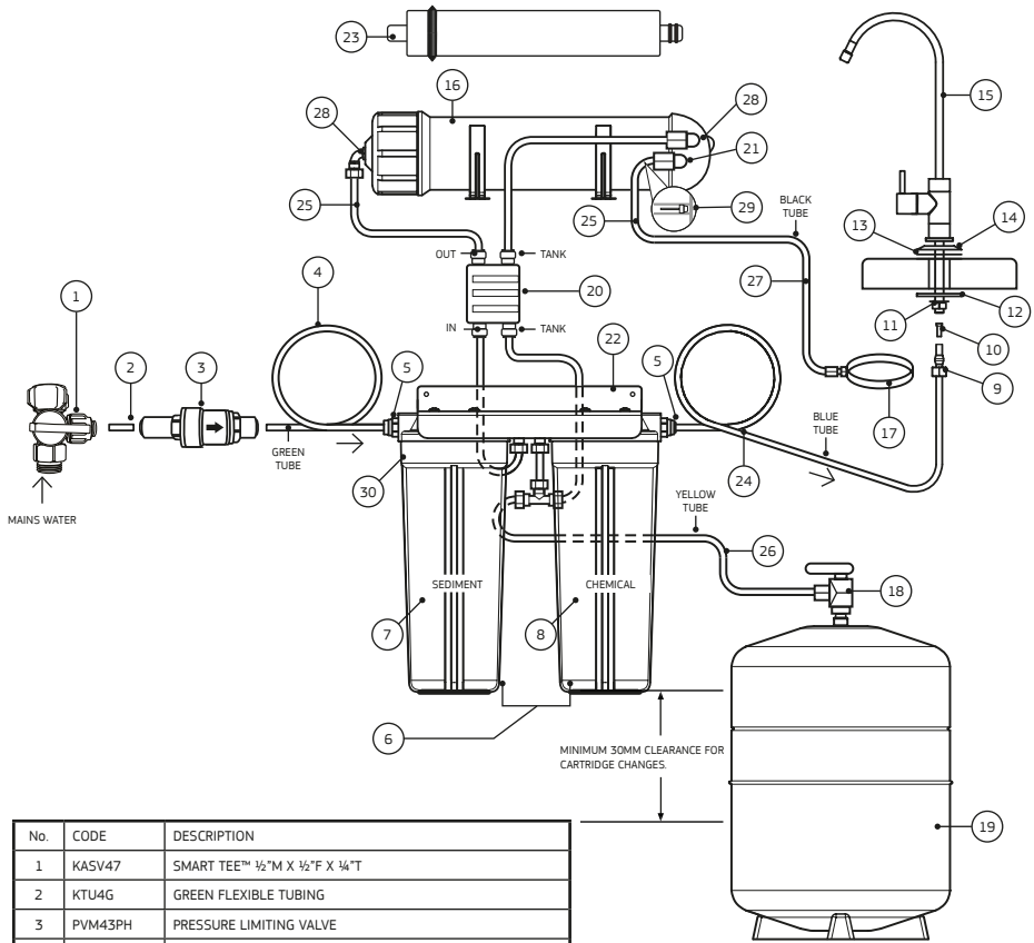
Figure 1 - Parts Diagram
